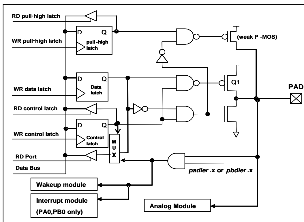
Fig. 8: Hardware diagram of IO buffer
