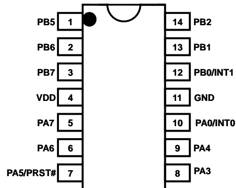
PMC153/PMS153 (SOP14 - 150mil) PMC153/PMS153 (DIP14 - 300mil)
